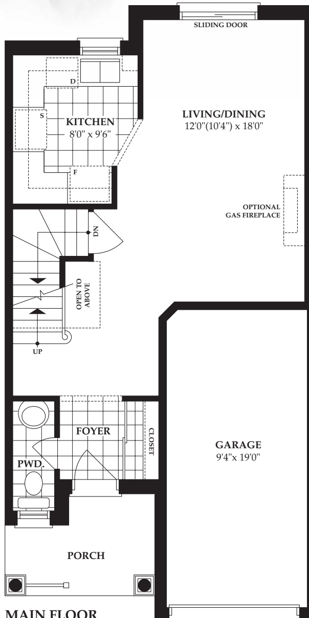
MAIN FLOOR ELEV. 3
