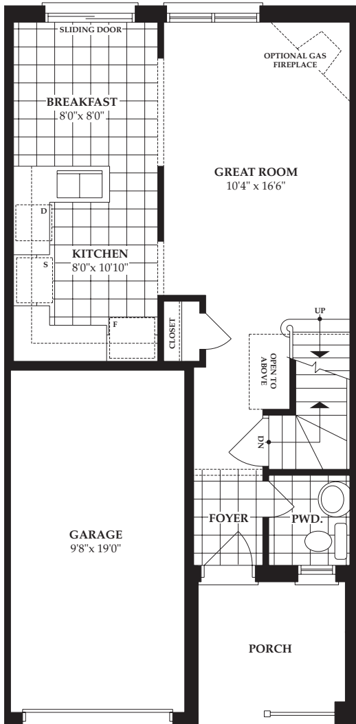
MAIN FLOOR ELEV. 2 (Rev.)
