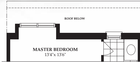
SECOND FLOOR PARTIAL PLAN - REAR (As Required)
