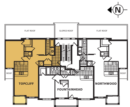
THIRD FLOOR - ELEV. 2
