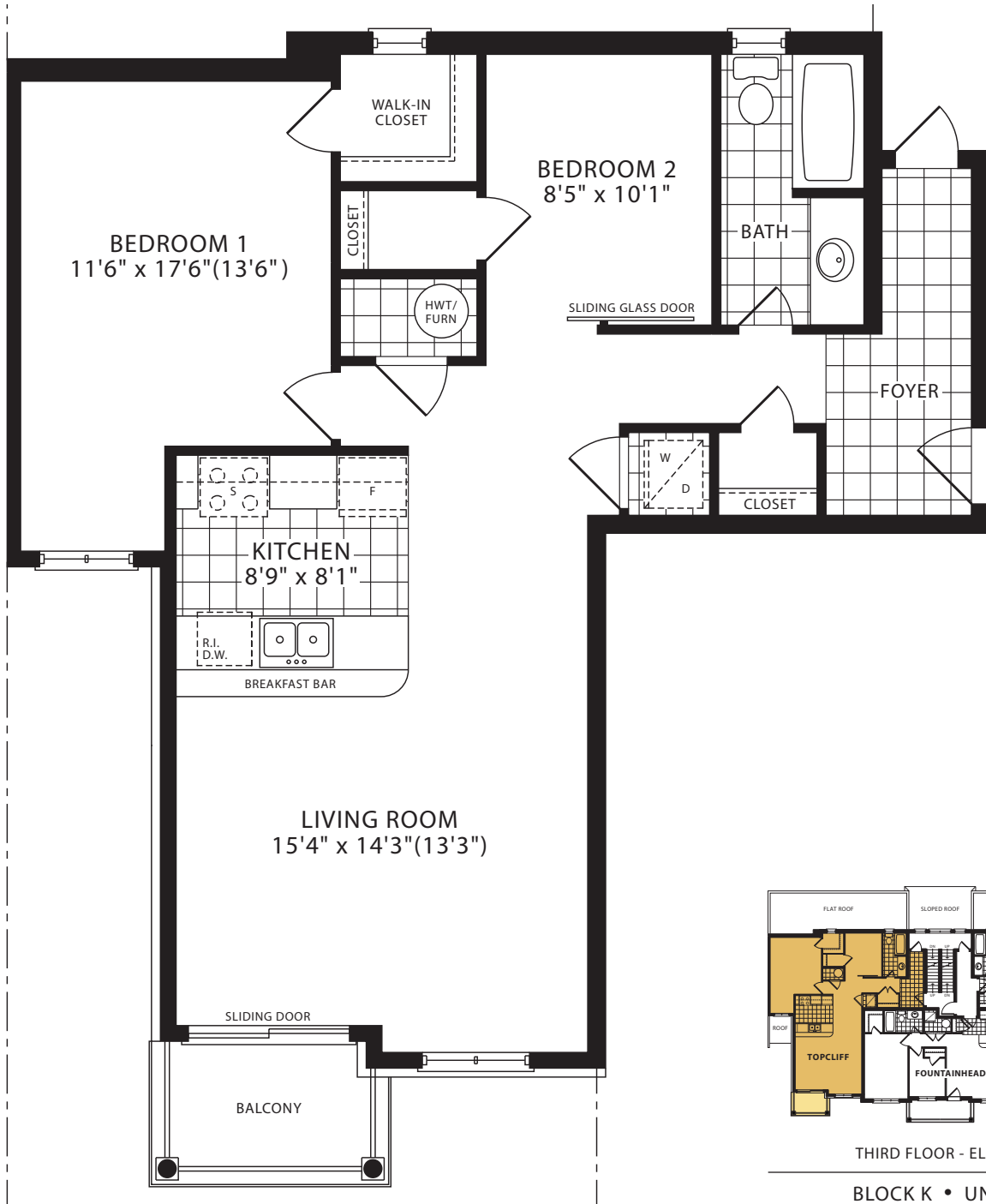
THIRD FLOOR ELEV. 2
