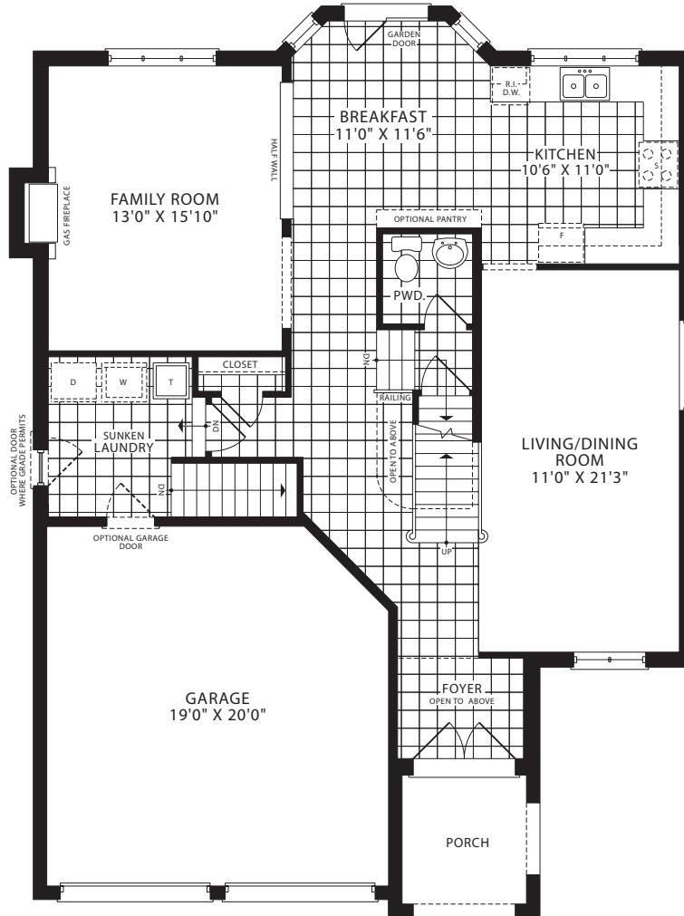
MAIN FLOOR ELEV. 1
